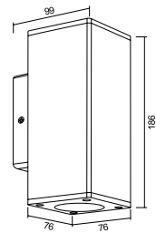
Up & Down Square
