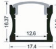
ML-073 2m Deep Surface Profile
