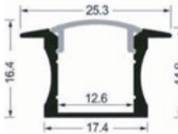
ML-074 2m Deep Recessed Profile
