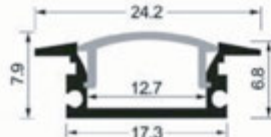
ML-072/082 2m Slim Recessed Profile
