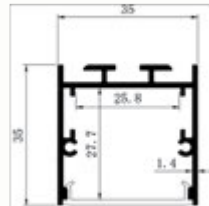
ML-035 3m Deep Surface Profile
